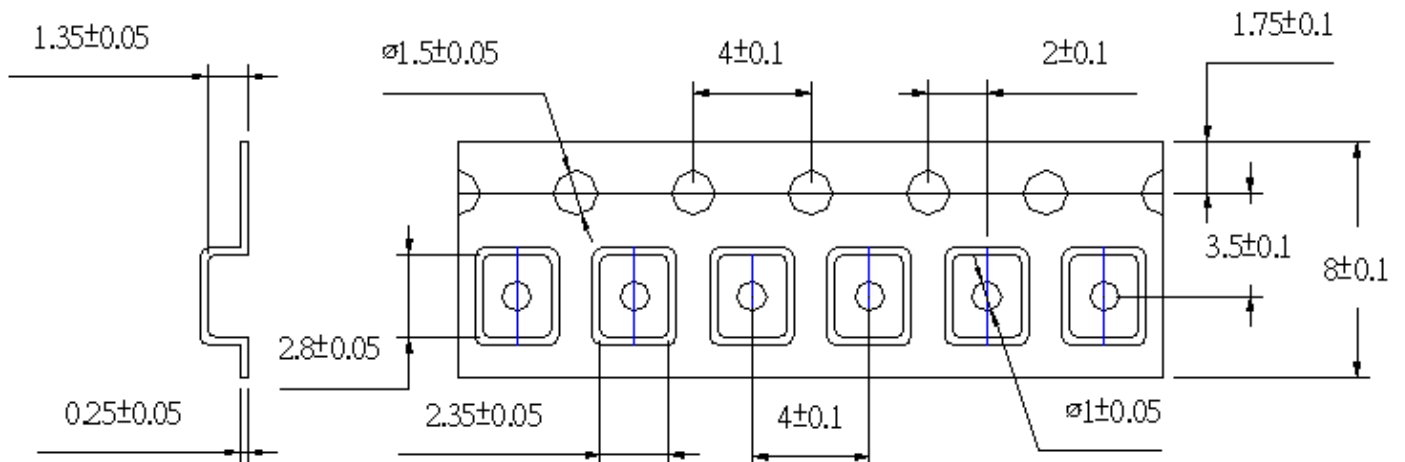
Taping dimension and tape direction, Leader ,Trailer, section dimension
